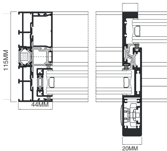
INTERLOCK HANDLE
