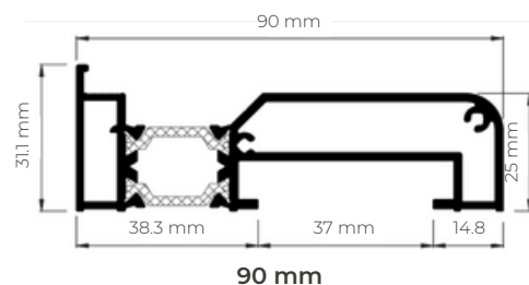
DRAINAGE SUBCILLS
