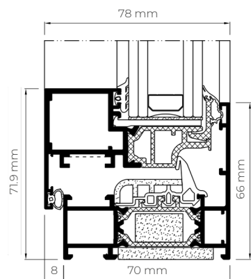
DRAINAGE SUBCILLS
