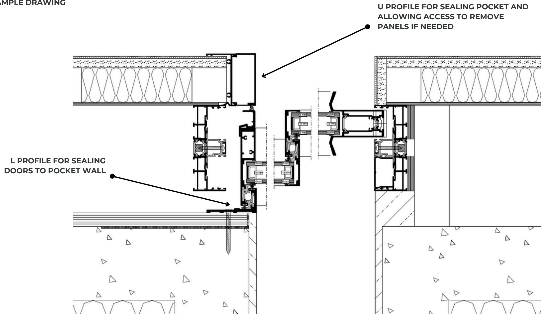
EXAMPLE DRAWING
