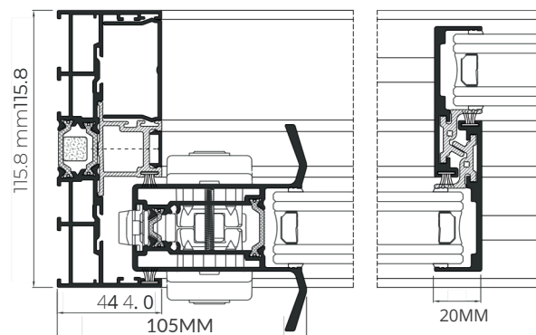
DOUBLE TRACK
